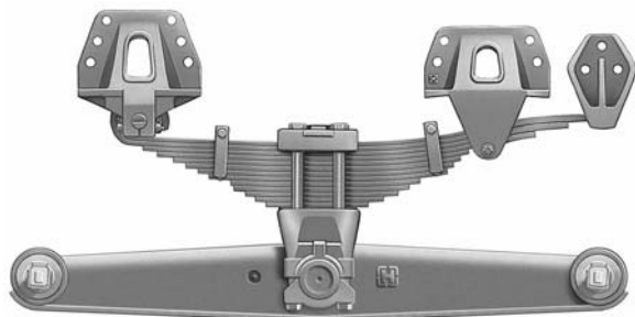
RTE Series with fabricated beam
