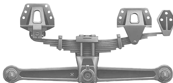
RTE Series with heavy-duty beam
